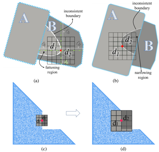
Fig. 7. (a) Fattening region detection and (b) narrowing region detection. d_1 and d_2 are two areas in the checking-window with different disparities. (c) and (d): size changing of the adaptive checking-window.
