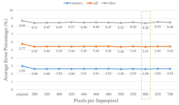
Fig. 6. Determination on superpixel size.
