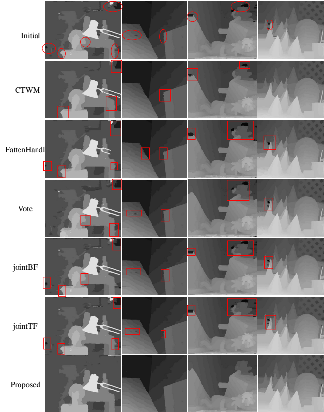
Fig. 11. Comparison with other refinement methods.
