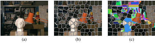
Fig. 5. (a) color image, (b) superpixels with SLIC, (c) segments with our method.
