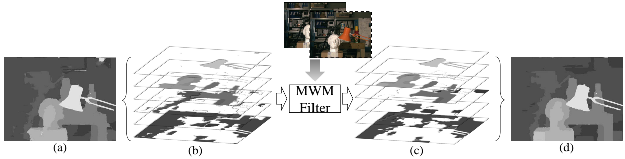
Fig. 8. Modified weighted median filtering process. (a) original disparity map, (b) disparity slices, (c) filtered disparity slices, (d) refined disparity map.
