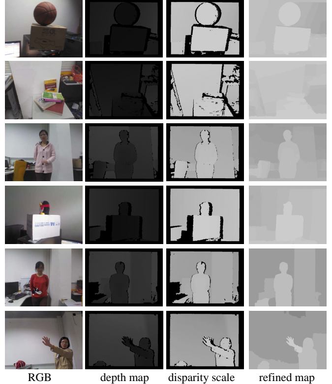
Fig. 12. Experimental results on depth maps obtained with Kinect.
