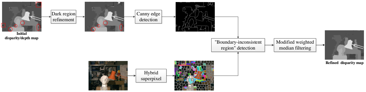
Fig. 1. Pipeline of the proposed disparity refinement method.
