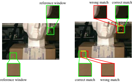
Fig. 3. Examples for fattening effect and narrowing effect. Left and right are the reference image and the target image respectively.
