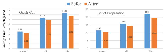
Fig. 10. Refinement results on Graph cut and Belief propagation.
