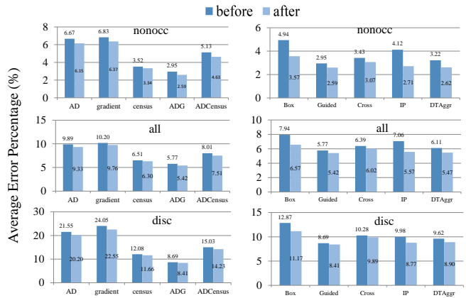
Fig. 9. Experimental evaluation on different cost measures and aggregation methods.
